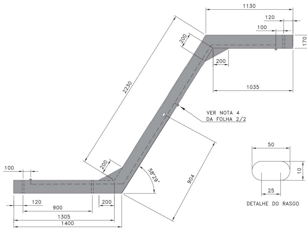
VISTA LATERAL – CRUZETA "Z"
