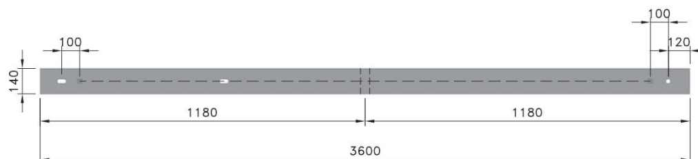
VISTA SUPERIOR – CRUZETA "I"
