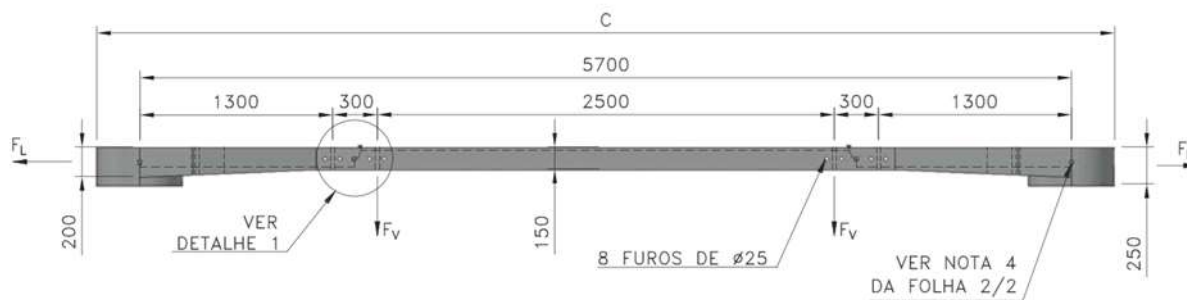
VISTA FRONTAL
