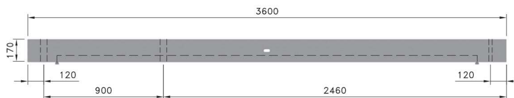
VISTA LATERAL – CRUZETA "I"
